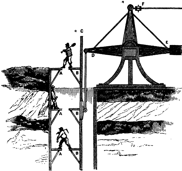
Fig. 165. "The Man Lifter," showing the fixed stages, or shelves, A, A, A, and the moving ones, B, B, B, attached to the rod, C, which is worked by the arm counterpoised by x. The pull is given at F. The man lifter is adopted at the Tresavean mine, which is 350 fathoms deep, and formerly occupied the miners one hour and a quarter to ascend by ladders placed nearly perpendicular.
